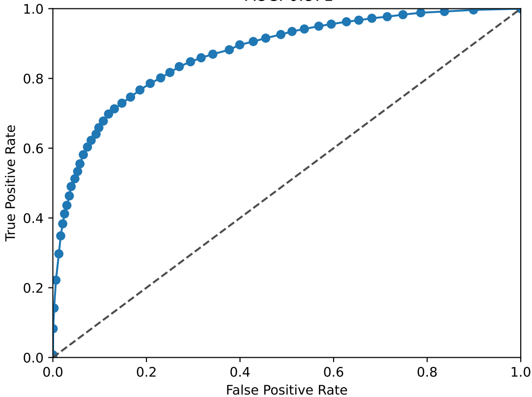
NFIB ROC Curve AUC: 0.871
