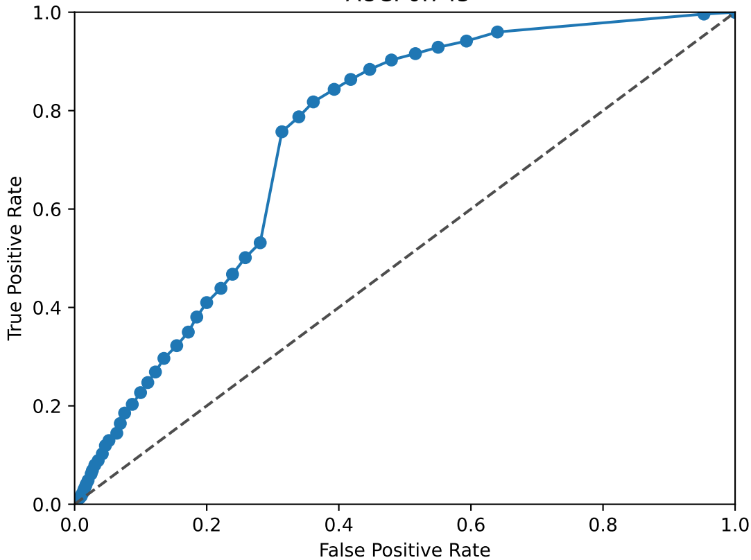
SIX1 ROC Curve AUC: 0.745
