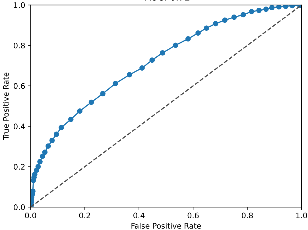
SIX4 ROC Curve AUC: 0.72
