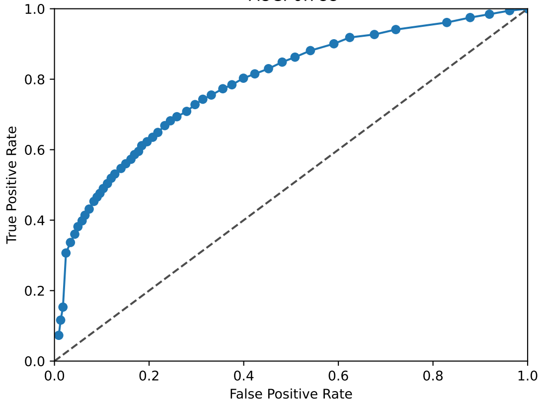
SMAD3 ROC Curve AUC: 0.788
