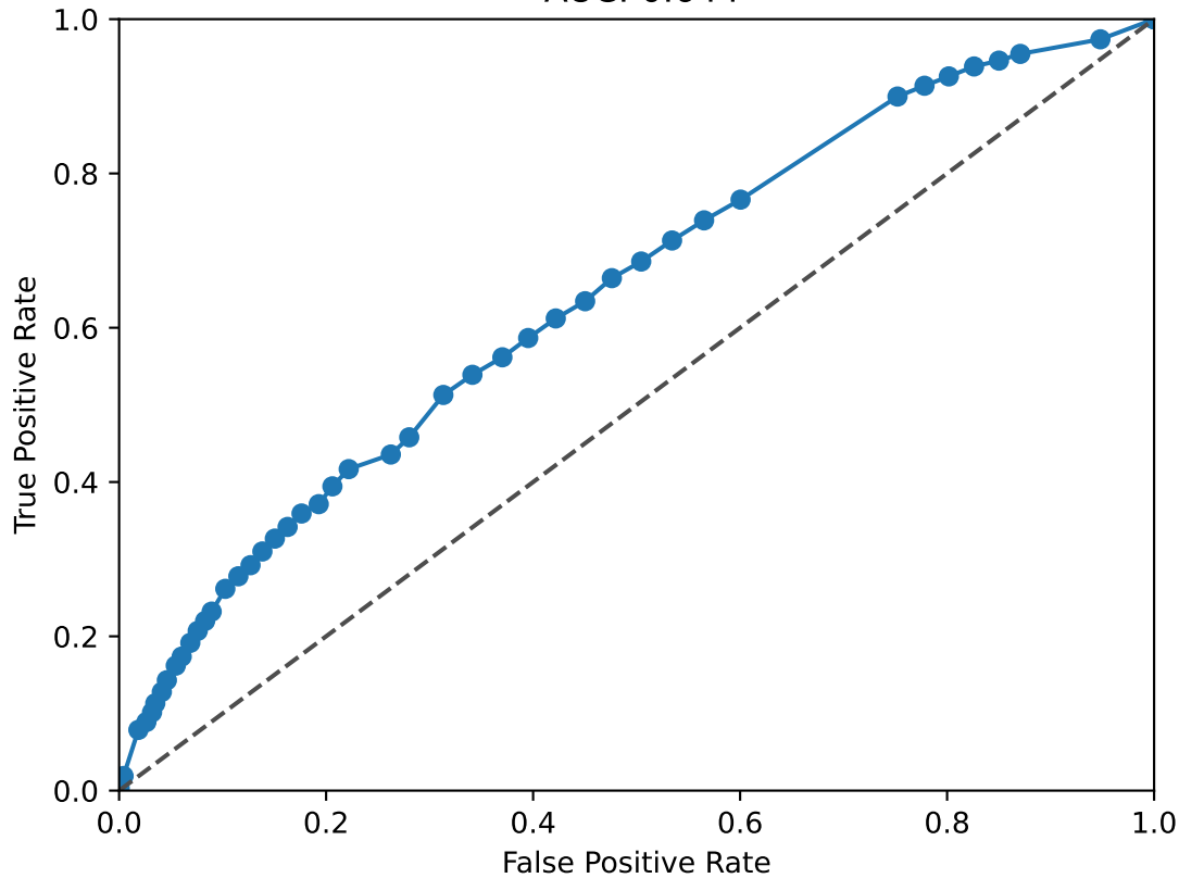
SOX11 ROC Curve AUC: 0.644
