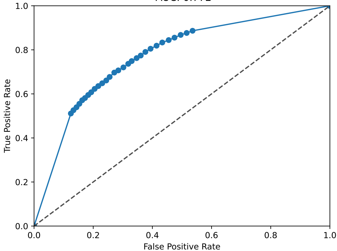
THR B ROC Curve AUC: 0.772
