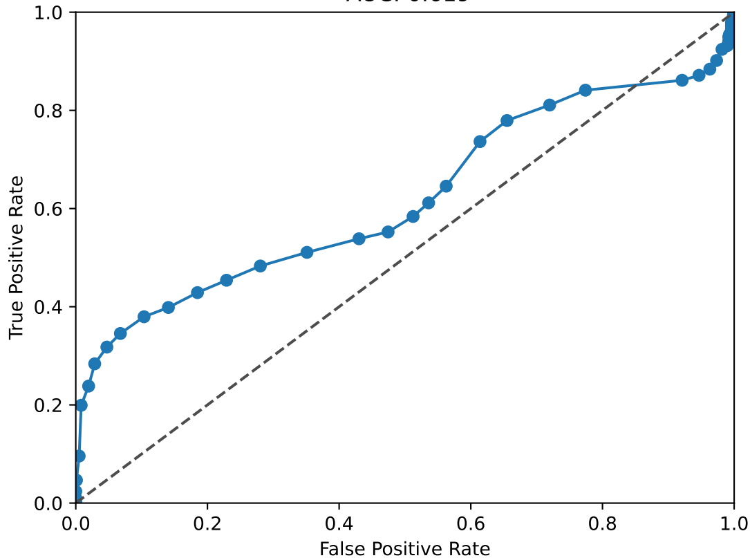
EGR1 ROC Curve AUC: 0.619
