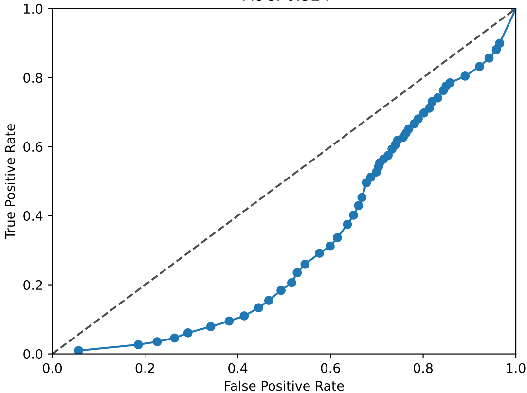
EPCAM ROC Curve AUC: 0.324
