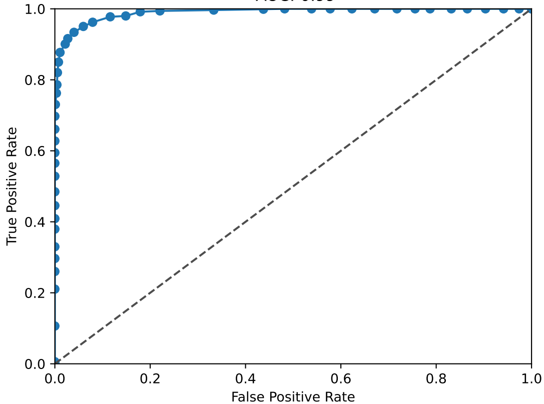
FOS ROC Curve AUC: 0.99
