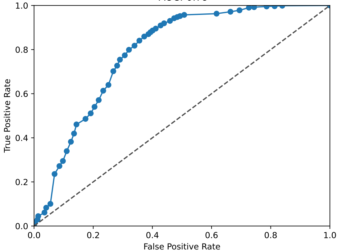
FOXO3 ROC Curve AUC: 0.79
