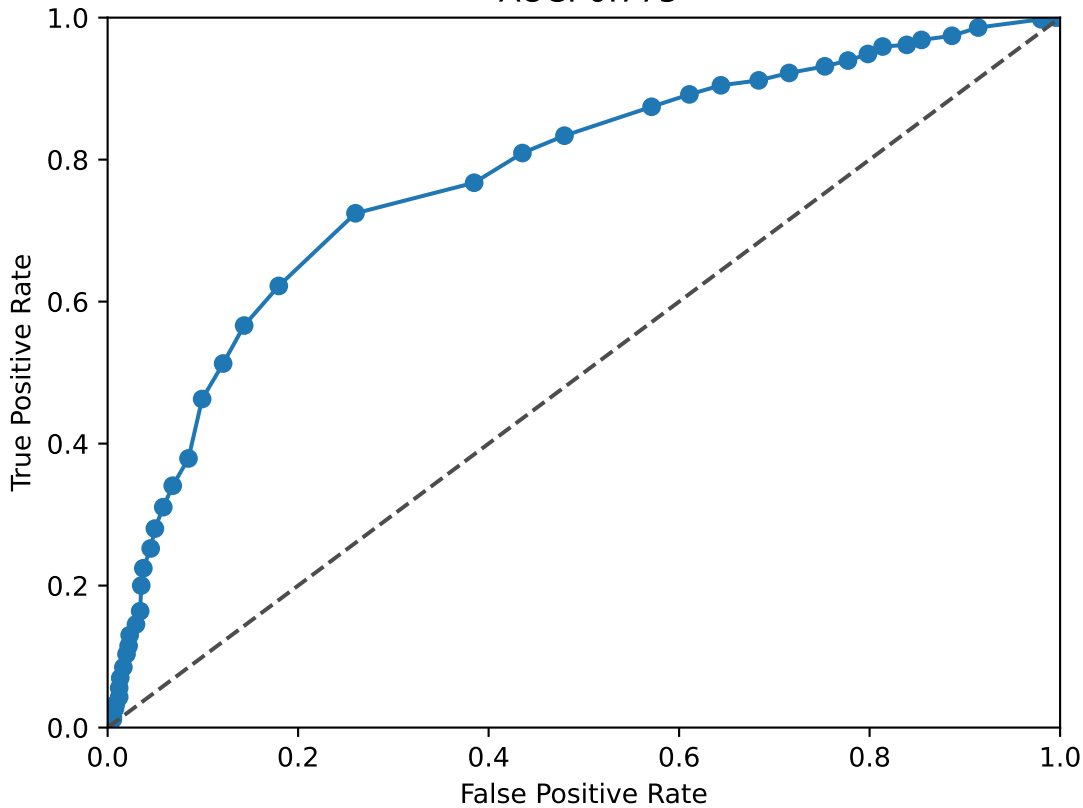
ICAM1 ROC Curve AUC: 0.775
