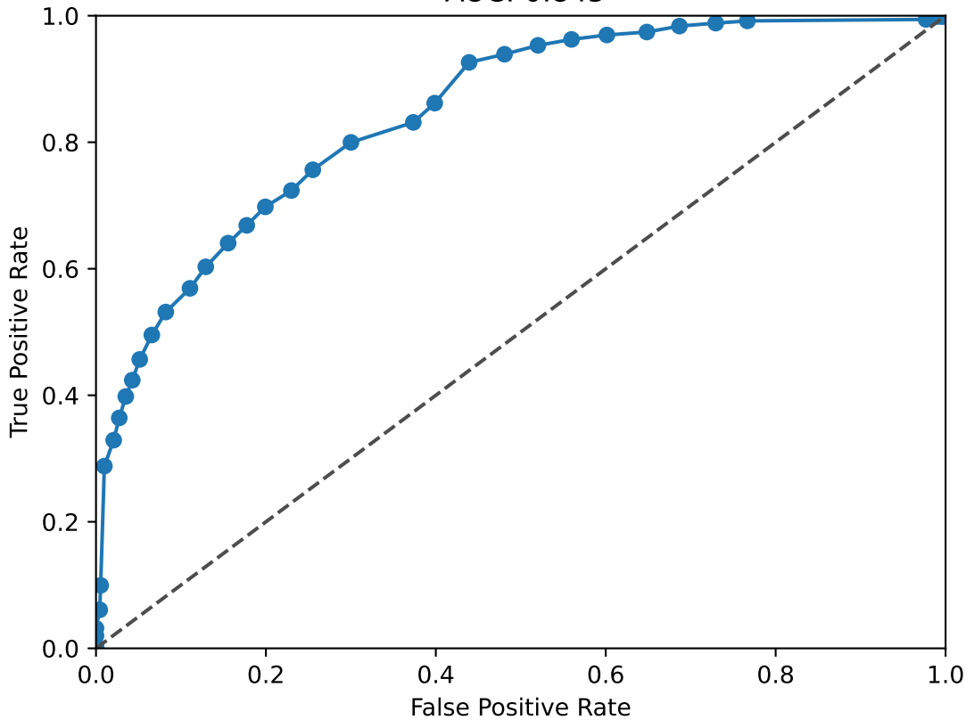
JUNB ROC Curve AUC: 0.845
