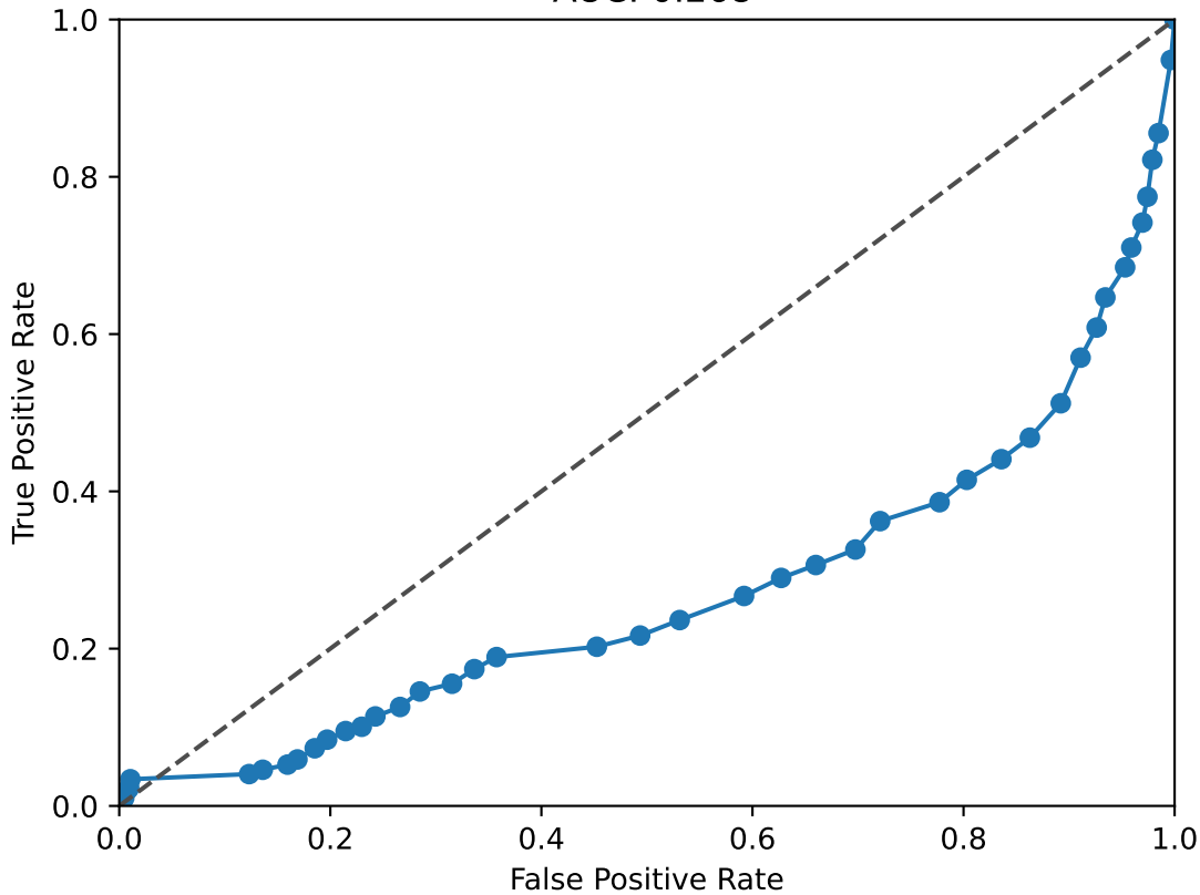
NFIX ROC Curve AUC: 0.268
