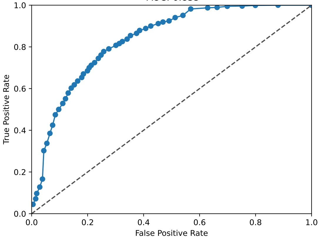
RORA_RORB ROC Curve AUC: 0.835
