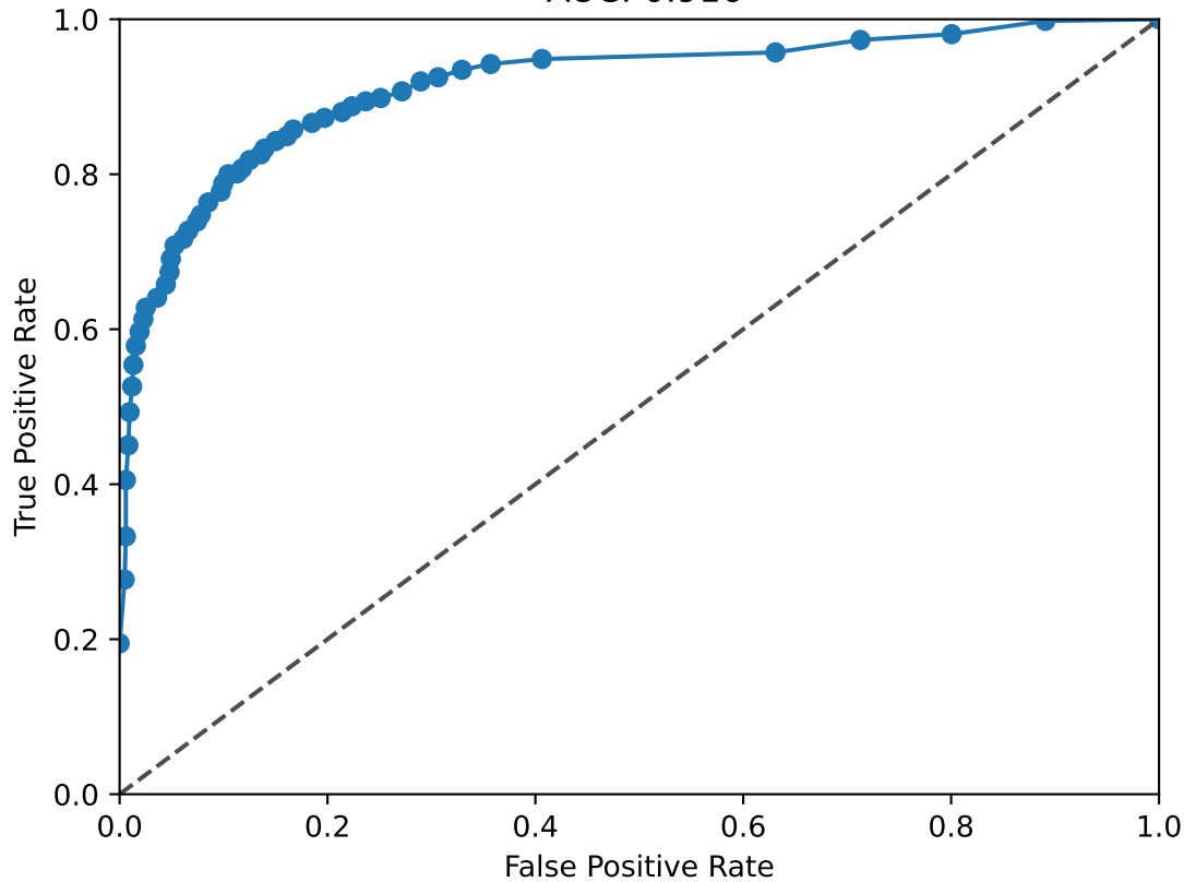
SMAD3 ROC Curve AUC: 0.916
