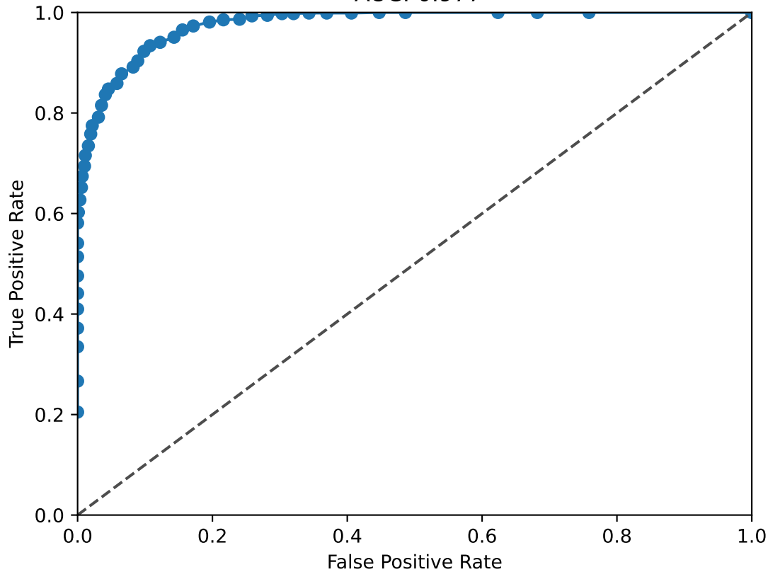
TCF7L1 ROC Curve AUC: 0.977
