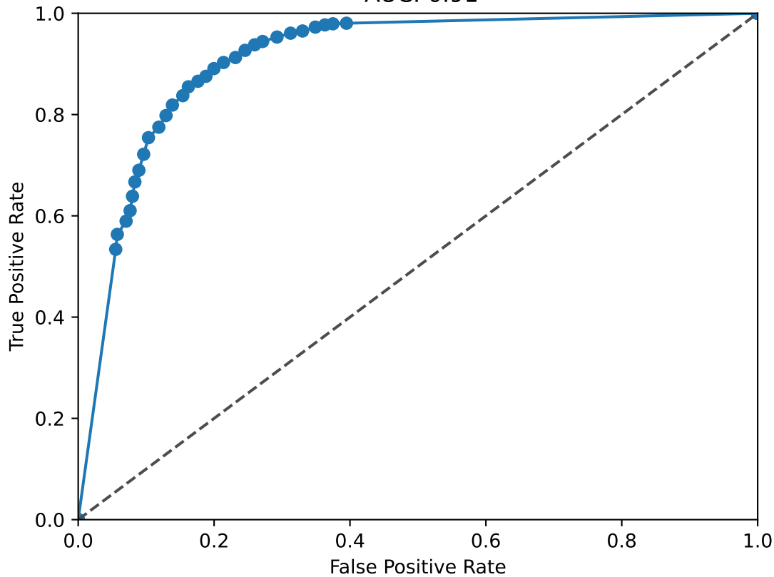
THR B ROC Curve AUC: 0.91
