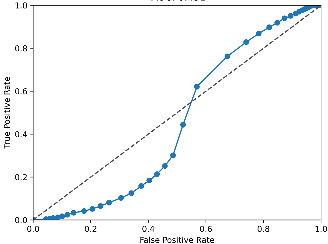
EGR1 ROC Curve AUC: 0.451
