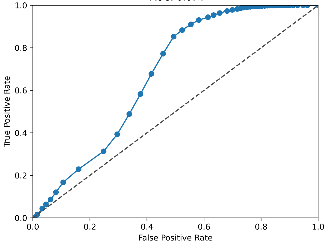
KMT2A ROC Curve AUC: 0.674
