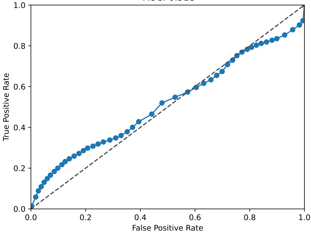
NFIA ROC Curve AUC: 0.518
