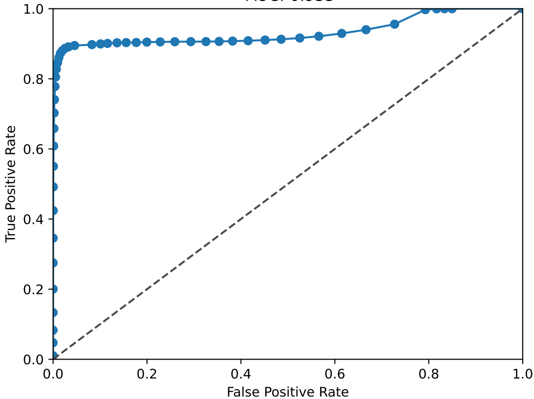
NFIB ROC Curve AUC: 0.933
