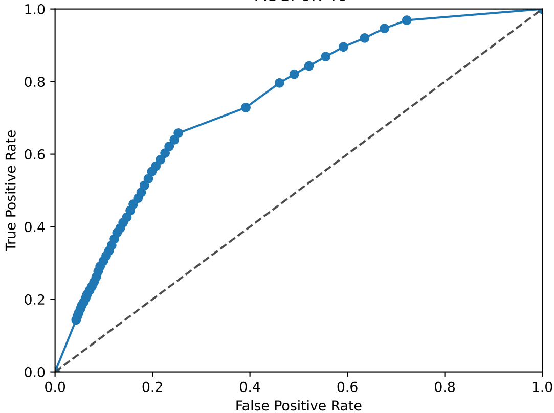
PROX1 ROC Curve AUC: 0.746
