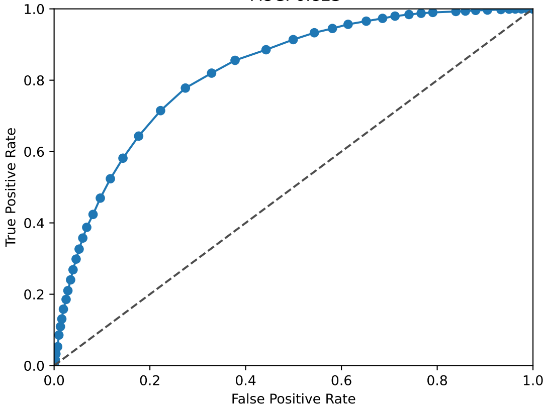
SIX4 ROC Curve AUC: 0.823
