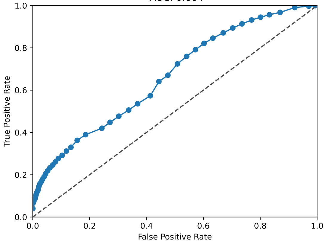
SMAD3 ROC Curve AUC: 0.664
