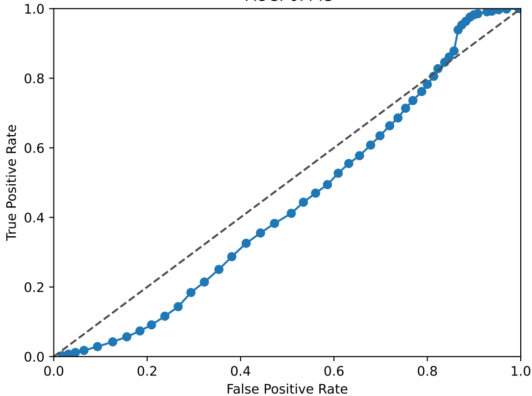
CUX2 ROC Curve AUC: 0.443
