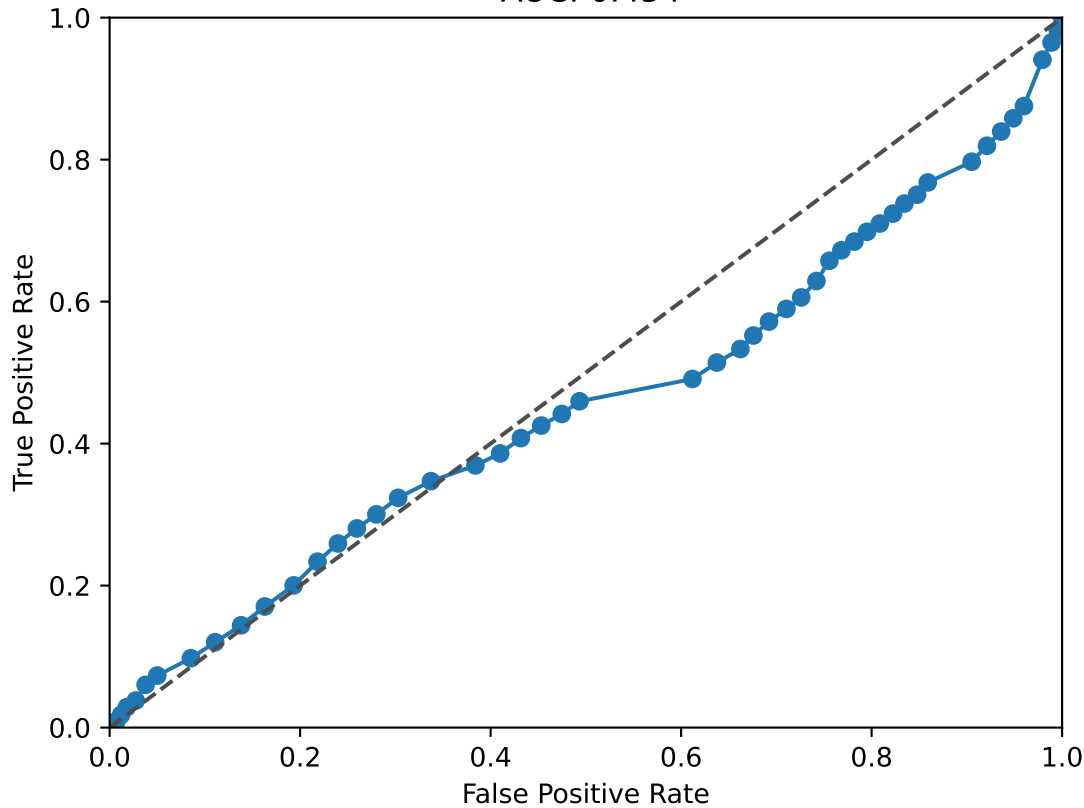
ETS1 ROC Curve AUC: 0.454
