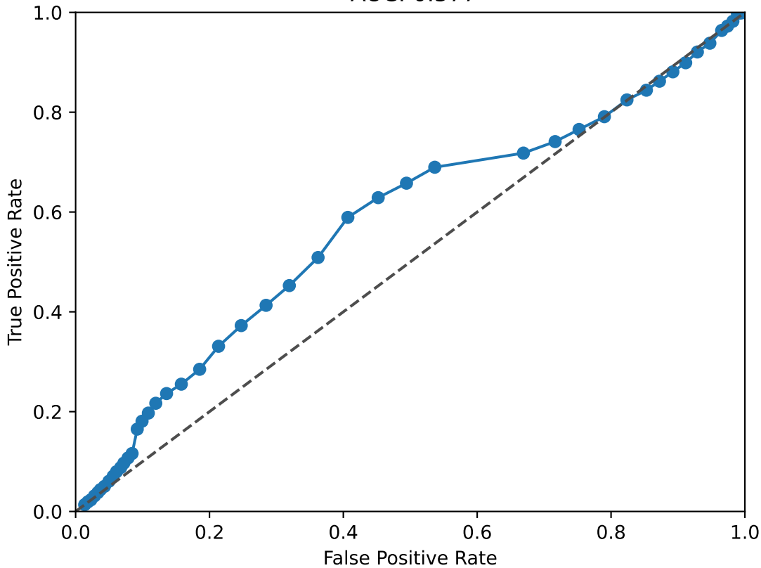
HES1 ROC Curve AUC: 0.577
