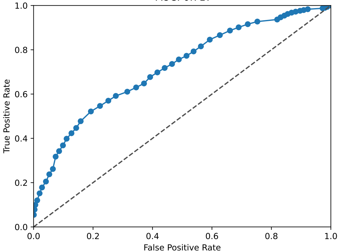
LMX1B ROC Curve AUC: 0.717
