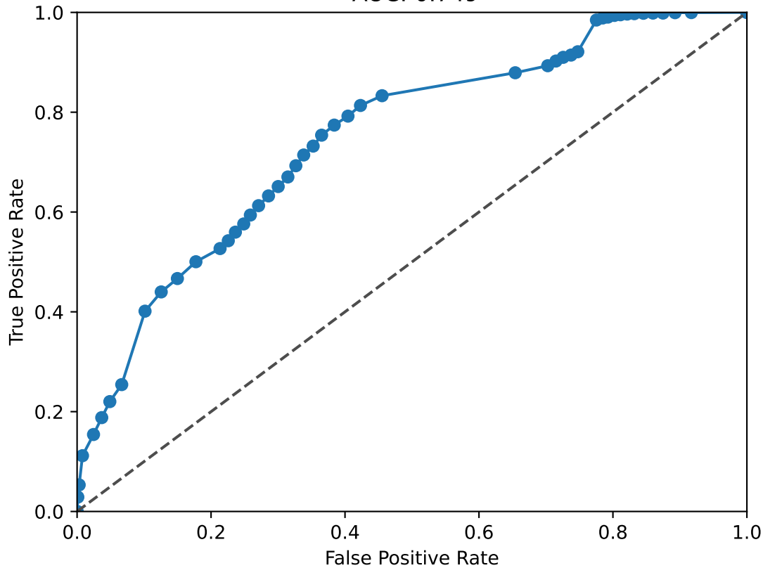
NFKB1 ROC Curve AUC: 0.749
