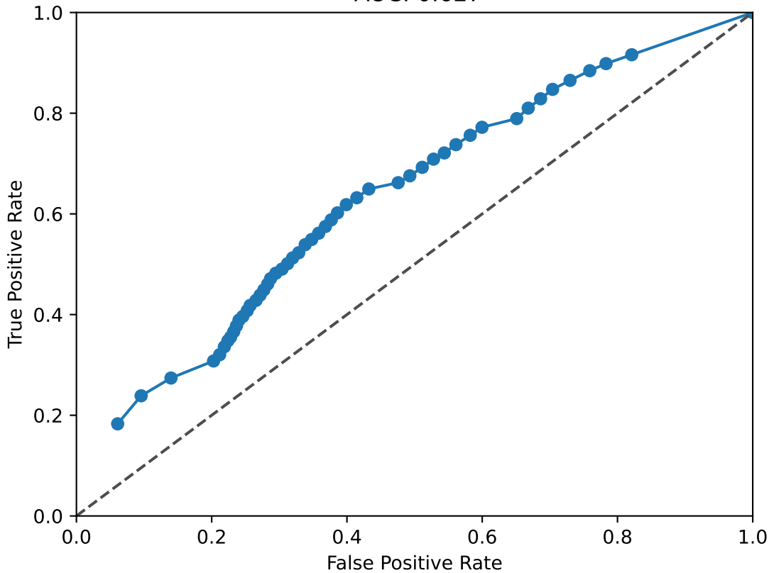
RORA_RORB ROC Curve AUC: 0.627
