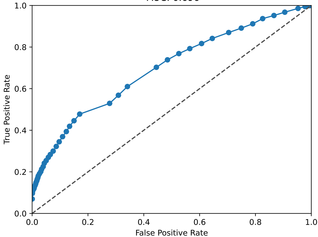
SMAD3 ROC Curve AUC: 0.696
