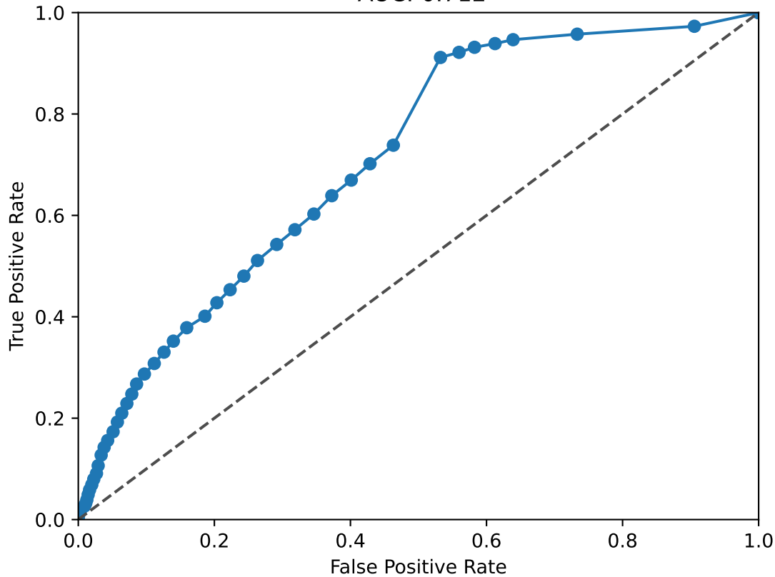
SOX11 ROC Curve AUC: 0.712
