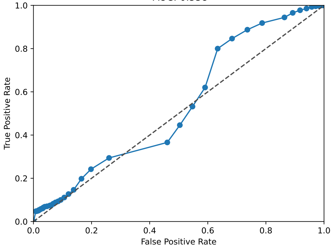
TCF7L1 ROC Curve AUC: 0.538
