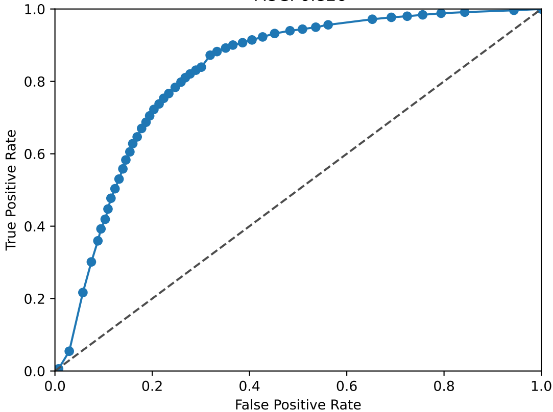
TEAD1 ROC Curve AUC: 0.826
