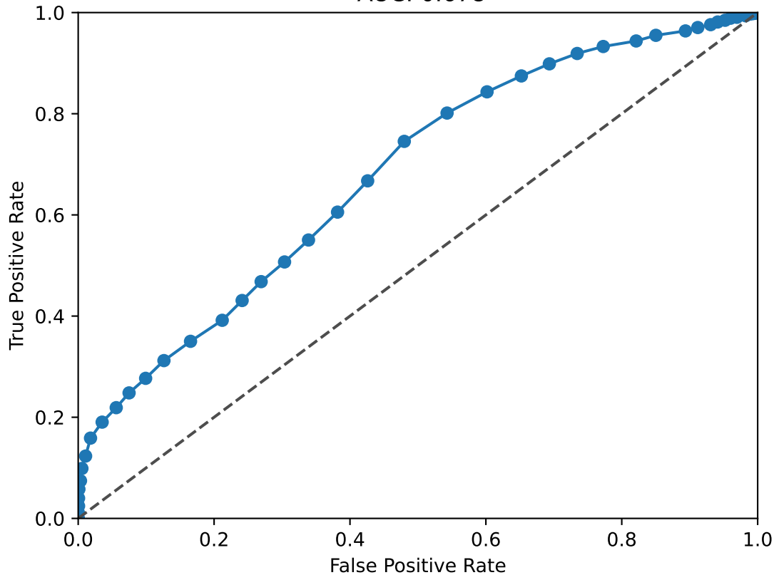
EGR1 ROC Curve AUC: 0.678
