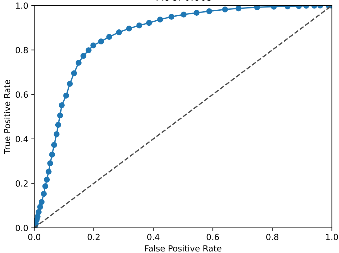
FOS ROC Curve AUC: 0.865
