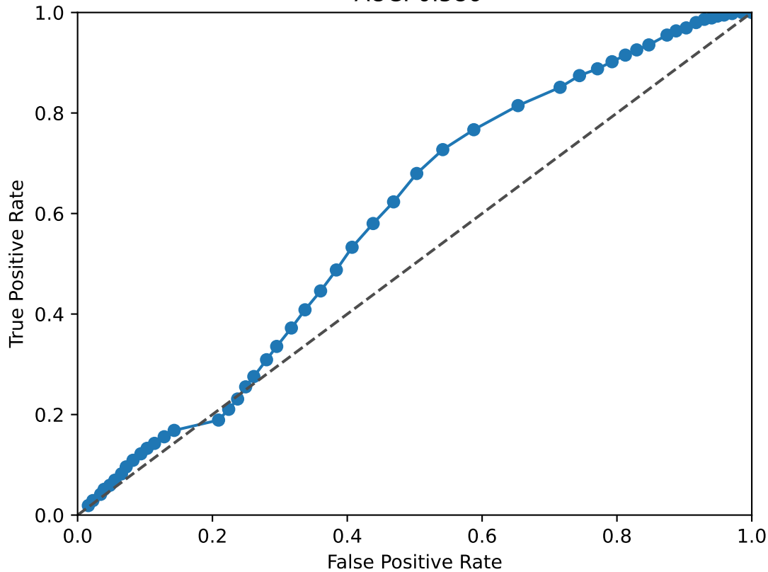
HES1 ROC Curve AUC: 0.586
