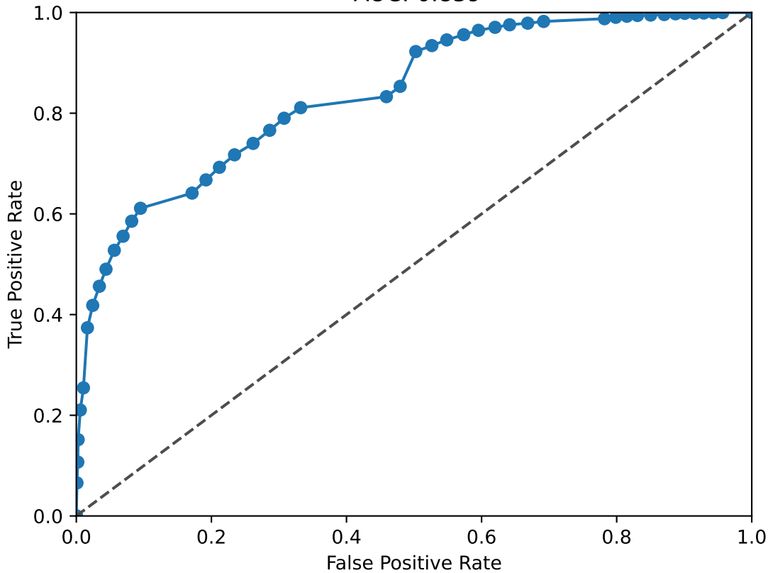
JUNB ROC Curve AUC: 0.839
