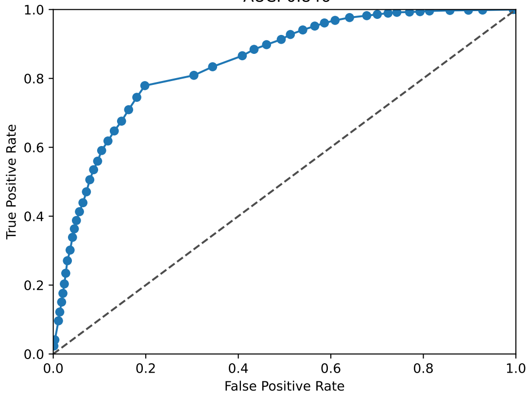
JUN ROC Curve AUC: 0.846
