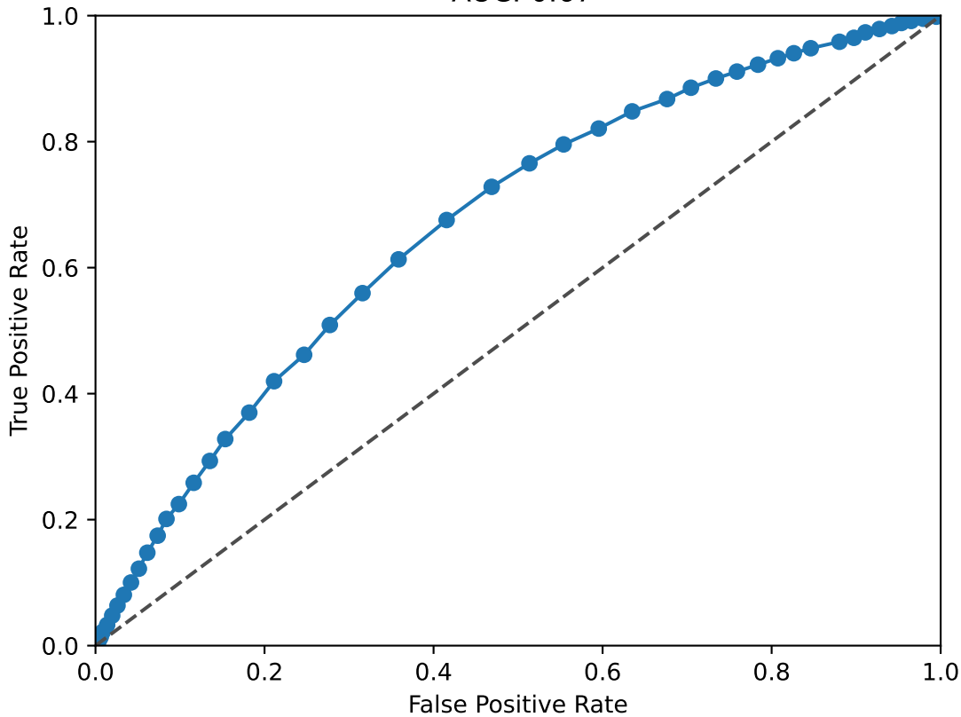
SIX4 ROC Curve AUC: 0.67
