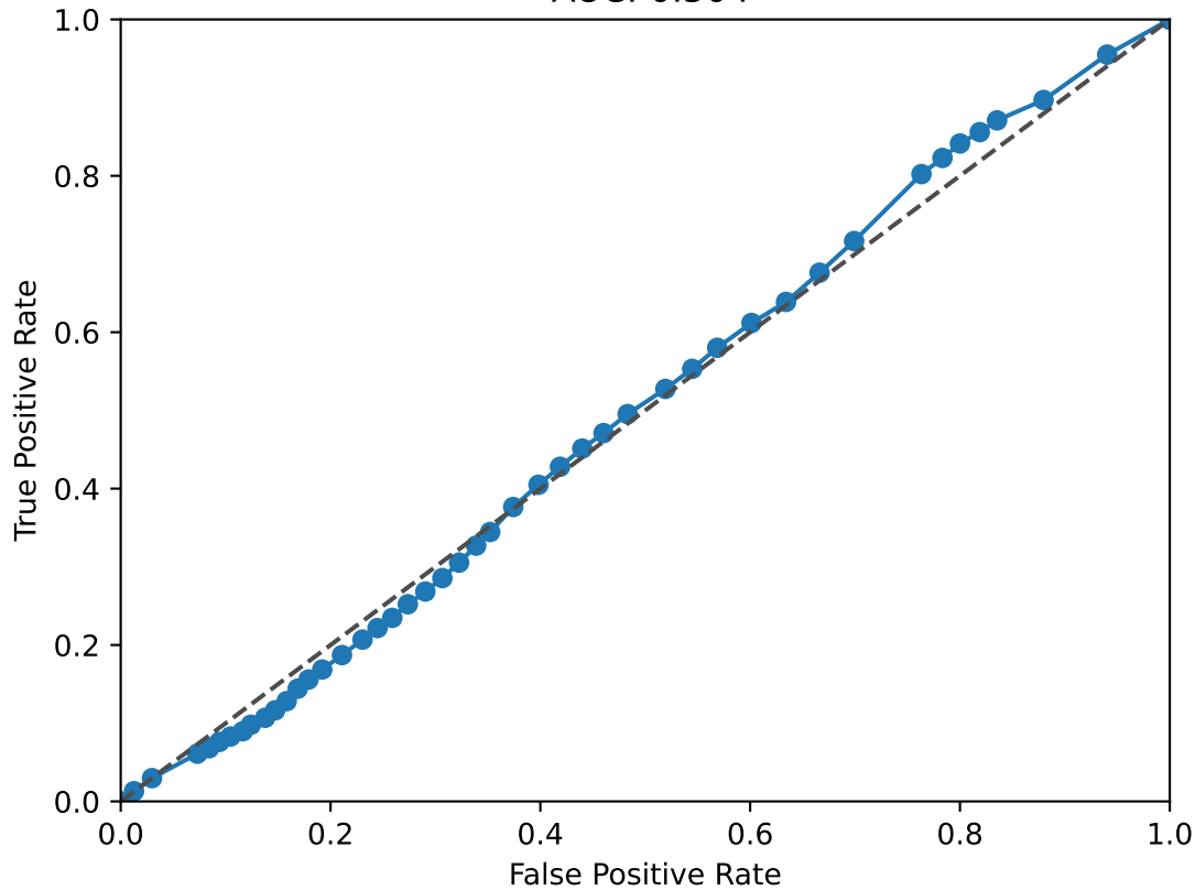
SOX11 ROC Curve AUC: 0.504
