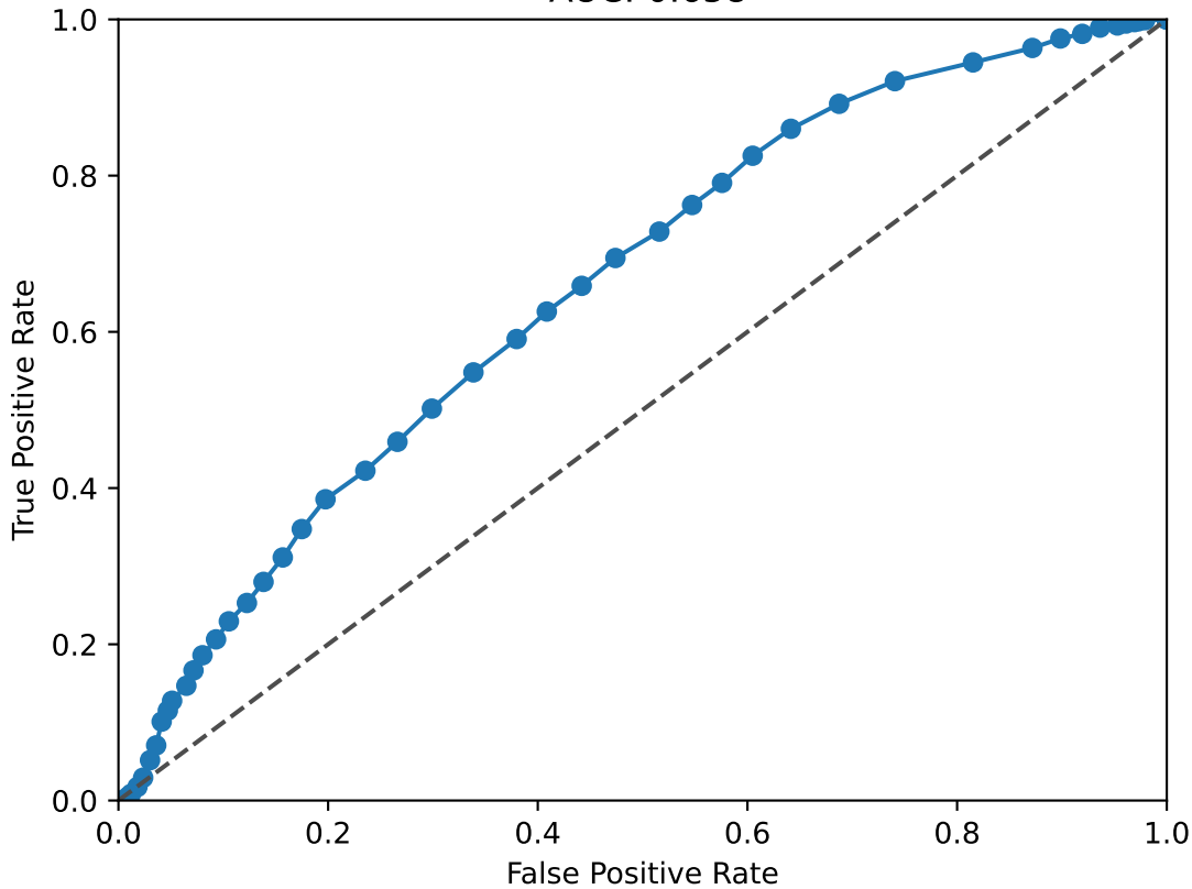
STAT2 ROC Curve AUC: 0.658
