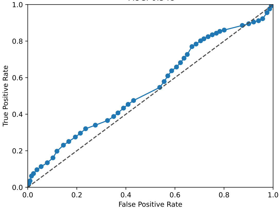
ETS1 ROC Curve AUC: 0.548
