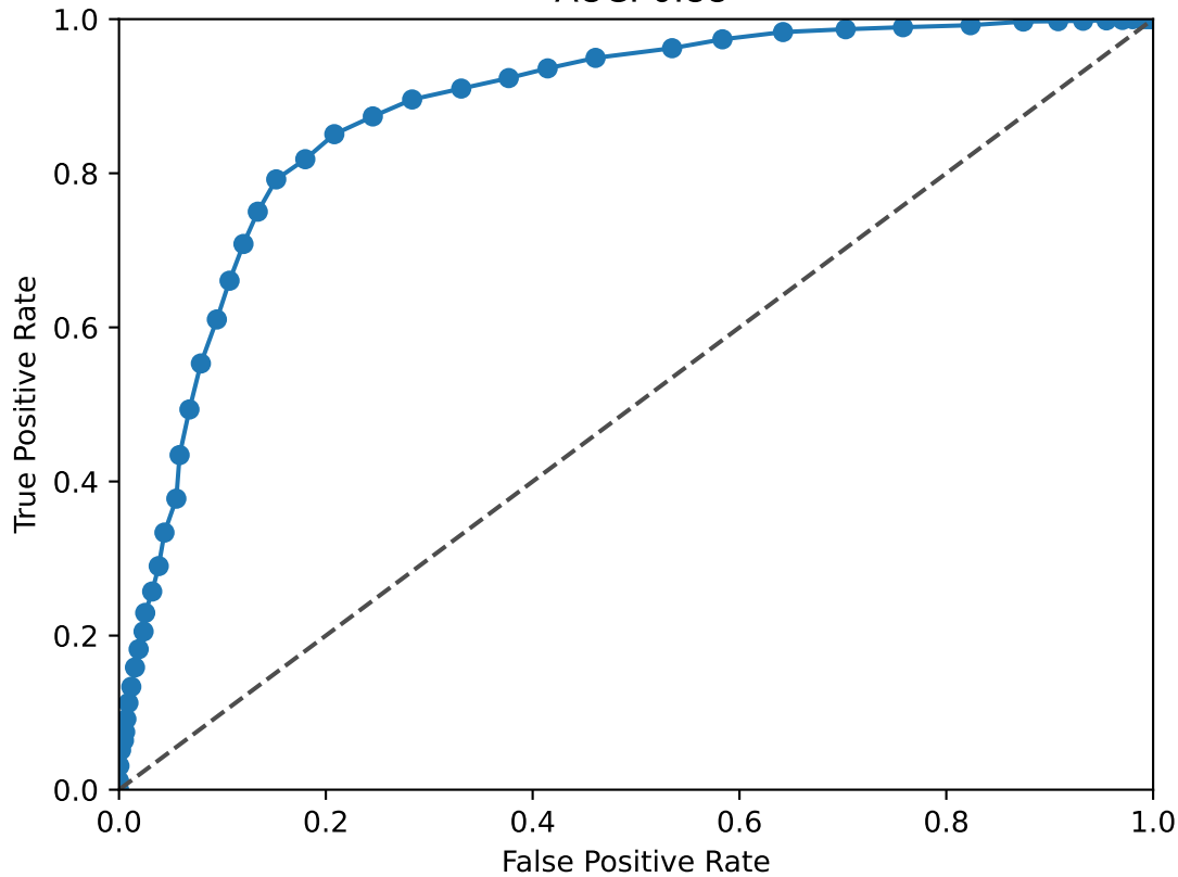
FOS ROC Curve AUC: 0.88
