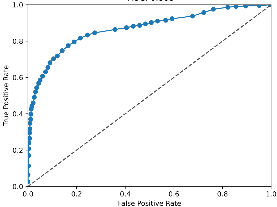
HSF2 ROC Curve AUC: 0.868
