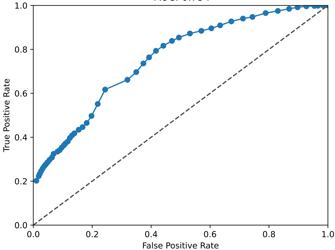
JUN ROC Curve AUC: 0.754
