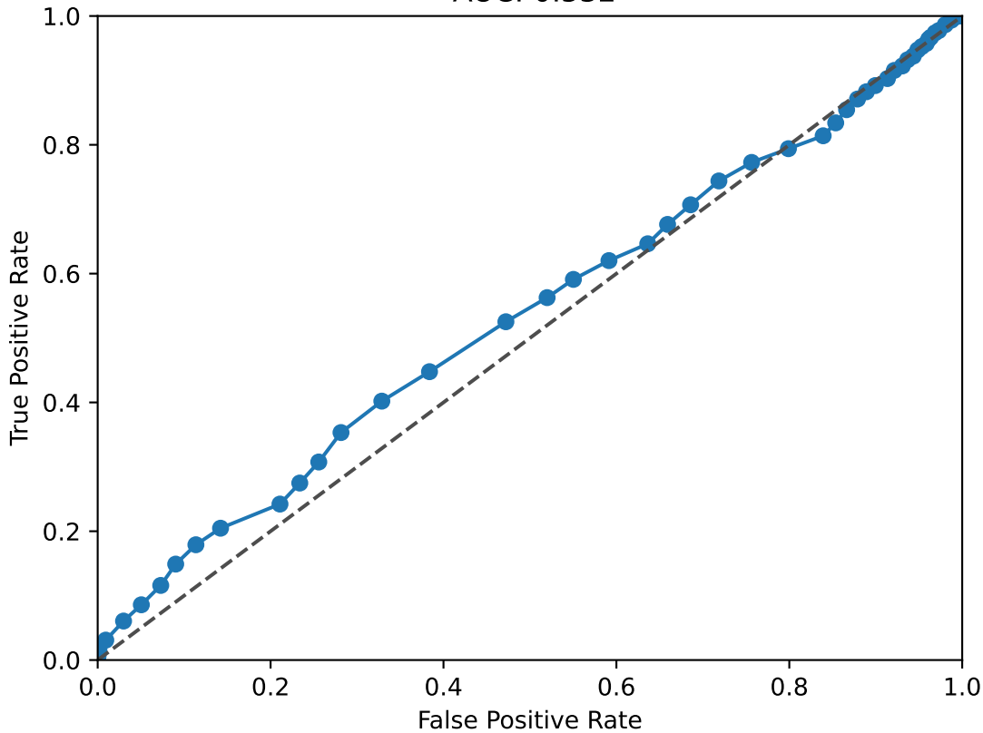
KMT2A ROC Curve AUC: 0.532
