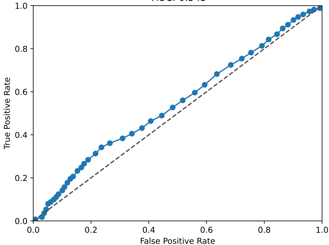
NCAM1 ROC Curve AUC: 0.545
