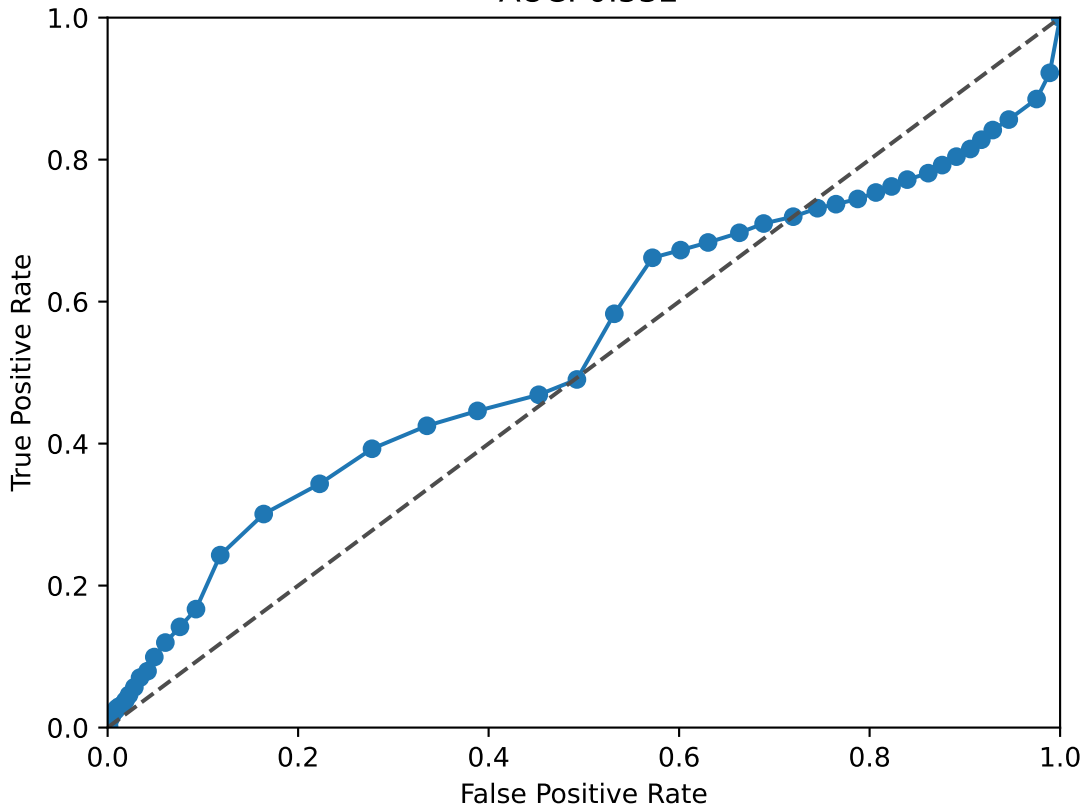
NFIA ROC Curve AUC: 0.532
