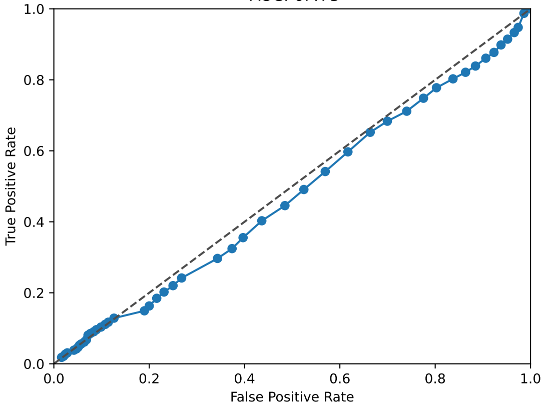
NFIX ROC Curve AUC: 0.473
